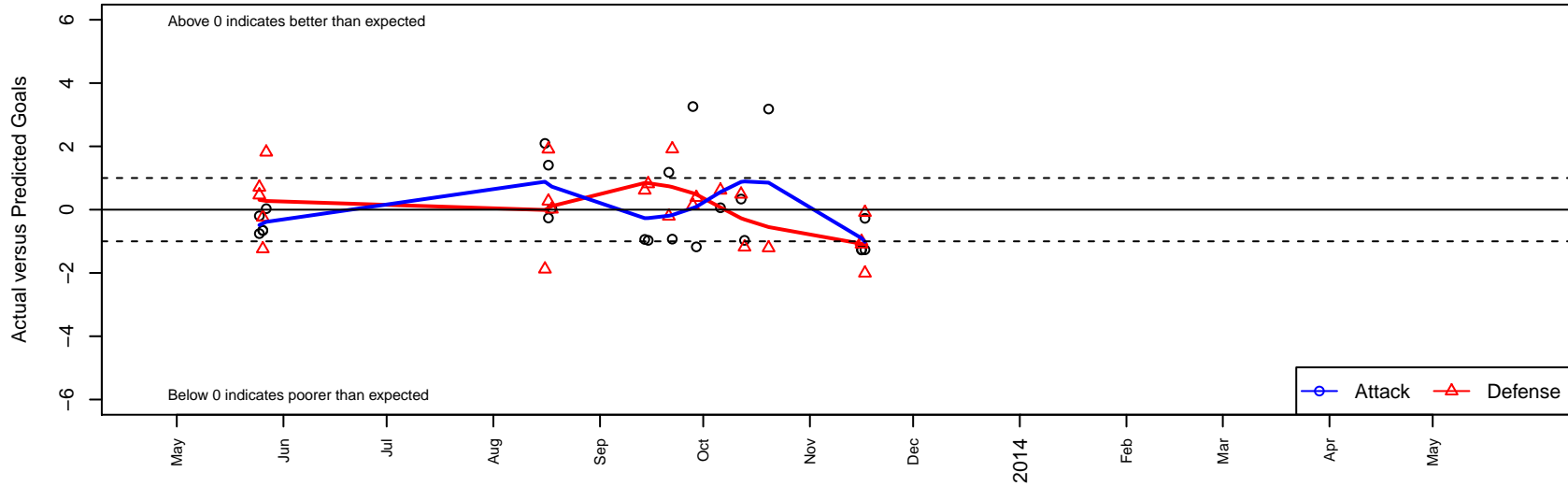
Ashland SC Fury G00 Dots are actual minus expected GF (blue circles) and GA (red triangles). Blue line is smoothed change in attack strength. Red is smoothed change in defense strength.
